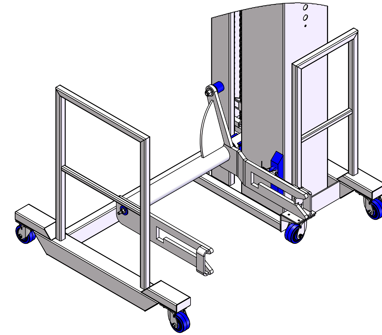
SHOWN WITH OPTIONAL PORTABLE CADDY ATTACHMENT
