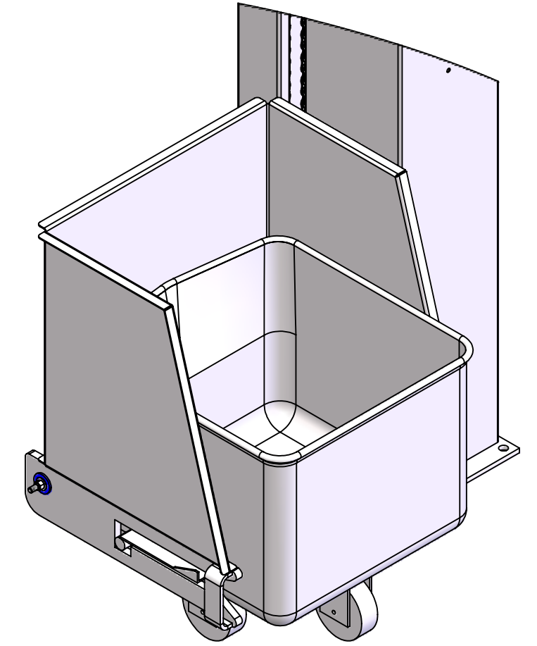
SHOWN WITH OPTIONAL CHUTE ATTACHMENT
